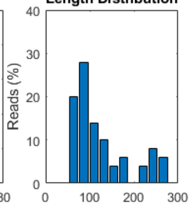
Length Distribution
