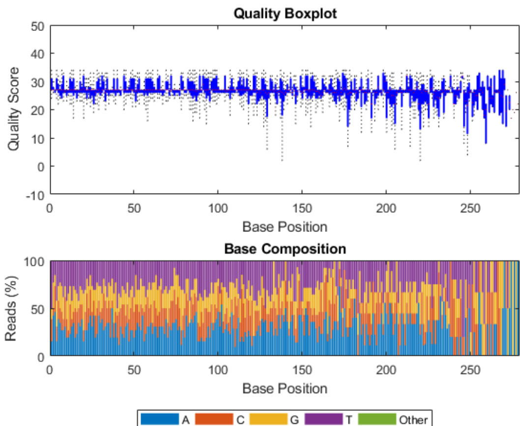
Quality Distribution
