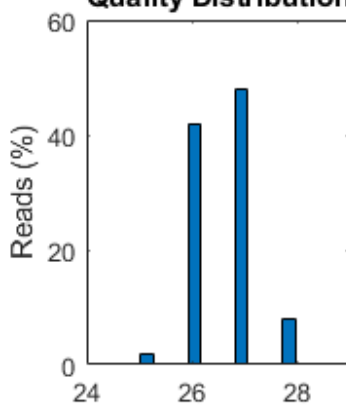
Quality Distribution
