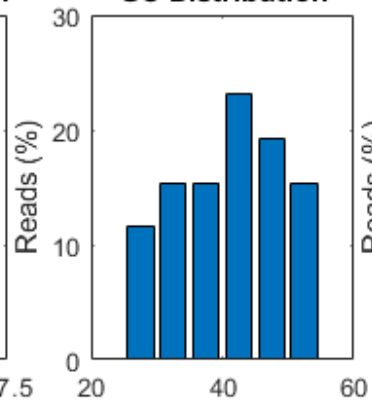
GC Distribution
