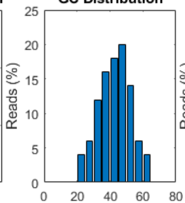
GC Distribution
