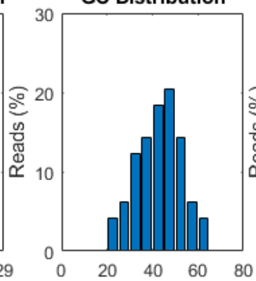
GC Distribution
