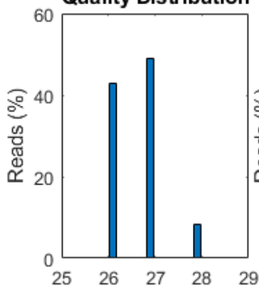
Quality Distribution
