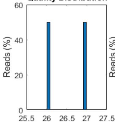
Quality Distribution
